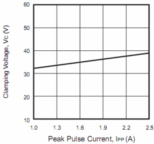
Fig.5 - TLP Measurement
