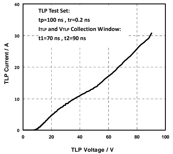
TLP Measurement
