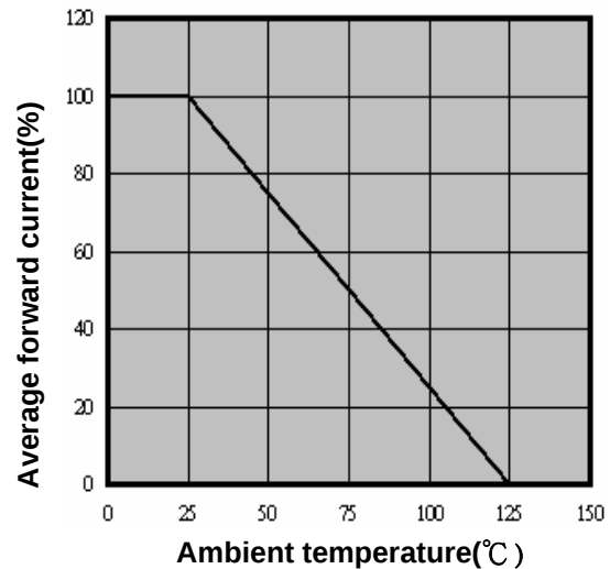
Fig.4-Current derating curve
