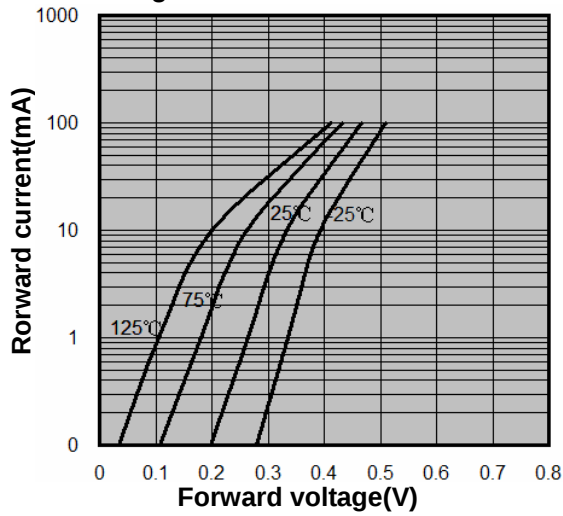
Fig.1-Forward characteristics
