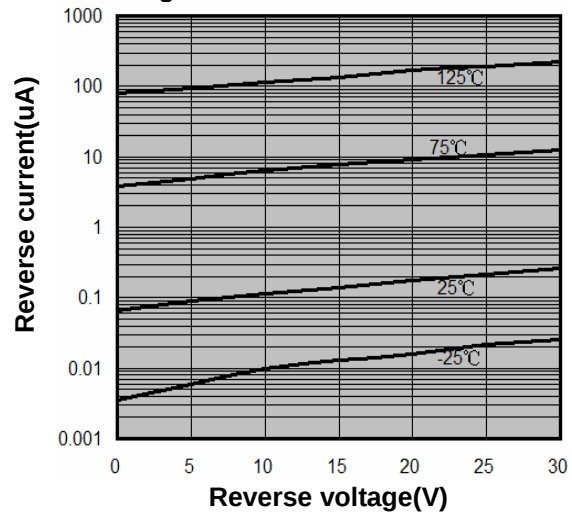
Fig.2-Reverse characteristics
