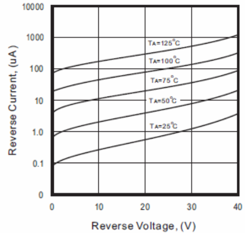
Fig.2 - Reverse Characteristics
